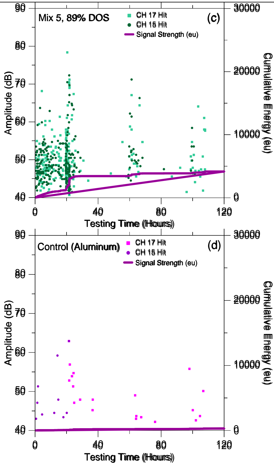
Figure 12 Acoustic Emission Hits and Cumulative Signal Strength (1eu=1nV·s) for (a) Fully Saturated (b) 94% Saturated and (c) 89% Saturated Concrete Undergoing Three Freeze-Thaw Cycles Compared to (D) an Aluminum Sample with No Freeze-Thaw Related Damage
