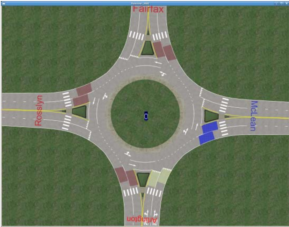
Figure A 3. Roundabout Marking – Type C – Exit Right
