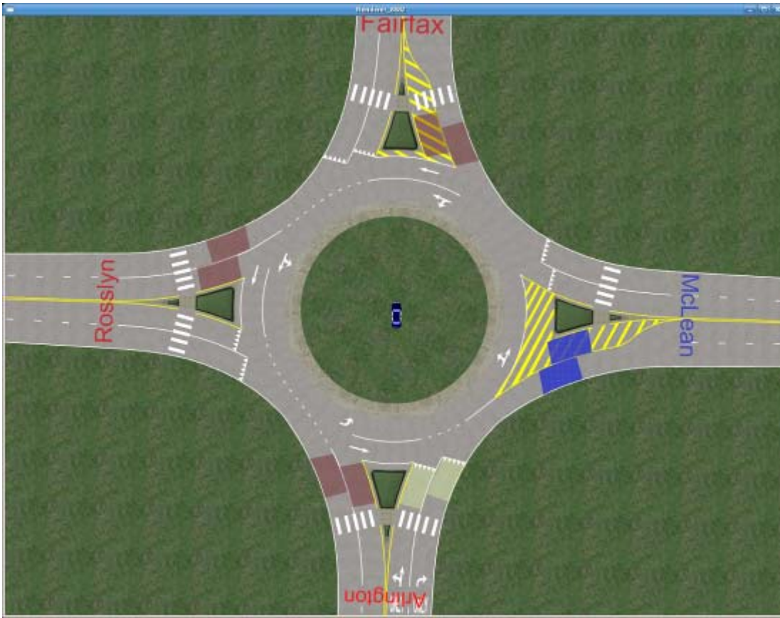
Figure A 4. Roundabout Marking – Type D – Exit Right
