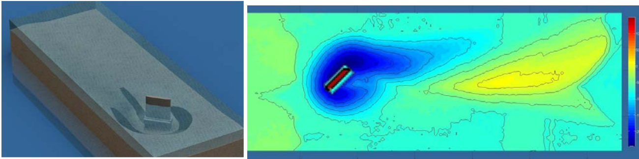
Figure 1 Measured scour hole in Tilting Flume
