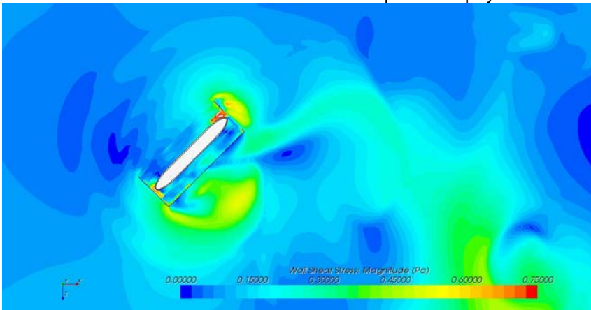
Figure 2 CFD bed shear result
