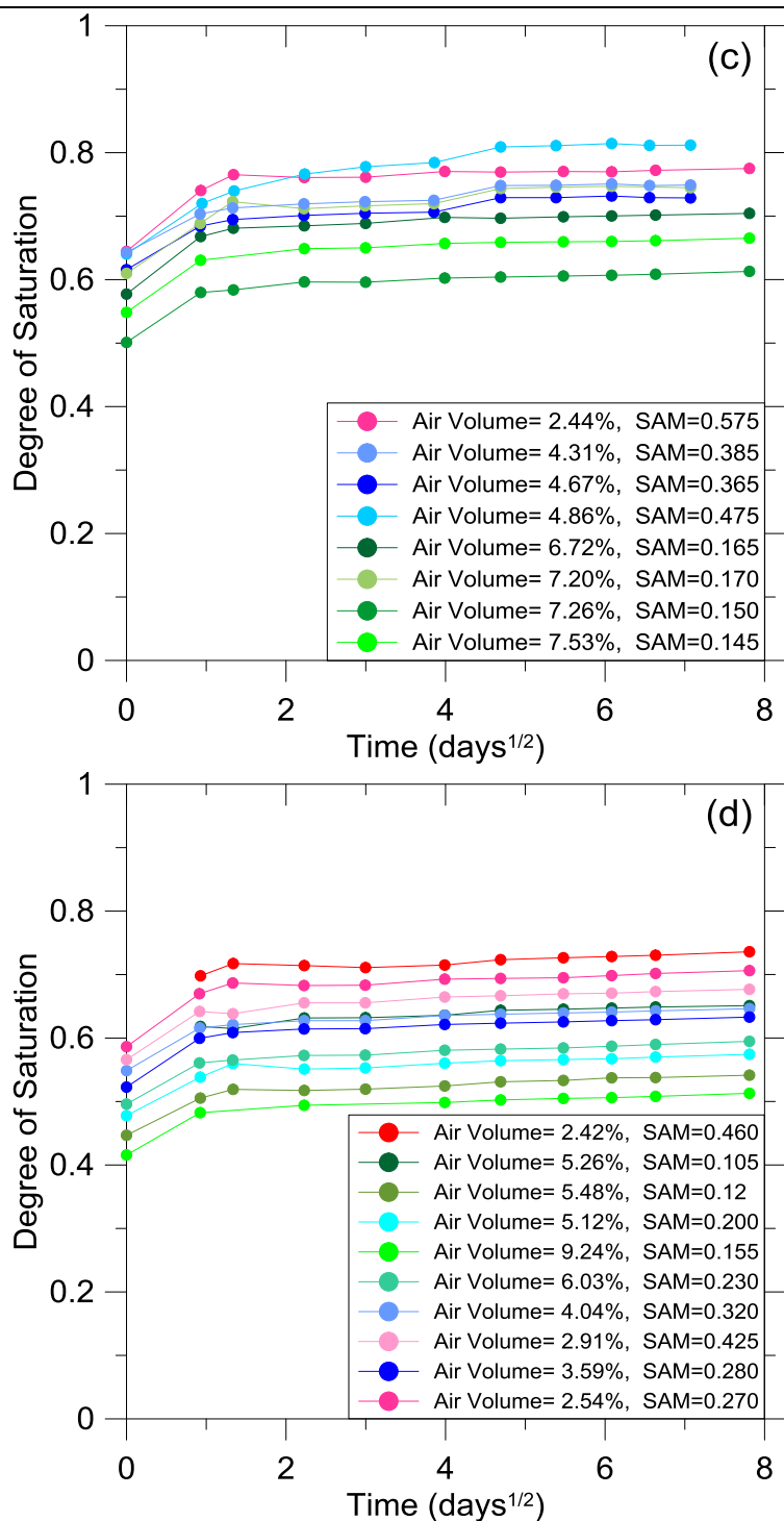
Figure 9 Degree of Saturation over Time for (a) Group 1, (b) Group 2, (c) Group 3 and (d) Group 4 Cylinders Submerged in Pore Solution
