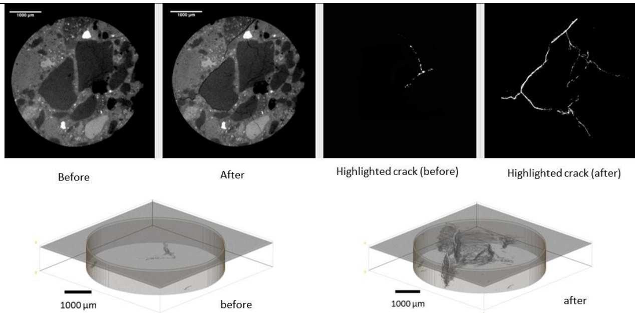
Figure 15 – An air entrained mortar sample shown both before and after a freeze thaw cycle. The highlighted cracks are shown from the cross sections. In addition, 3D data sets are shown of the crack distribution both before and after the freeze thaw cycle. The data was obtained with X-ray mCT.
