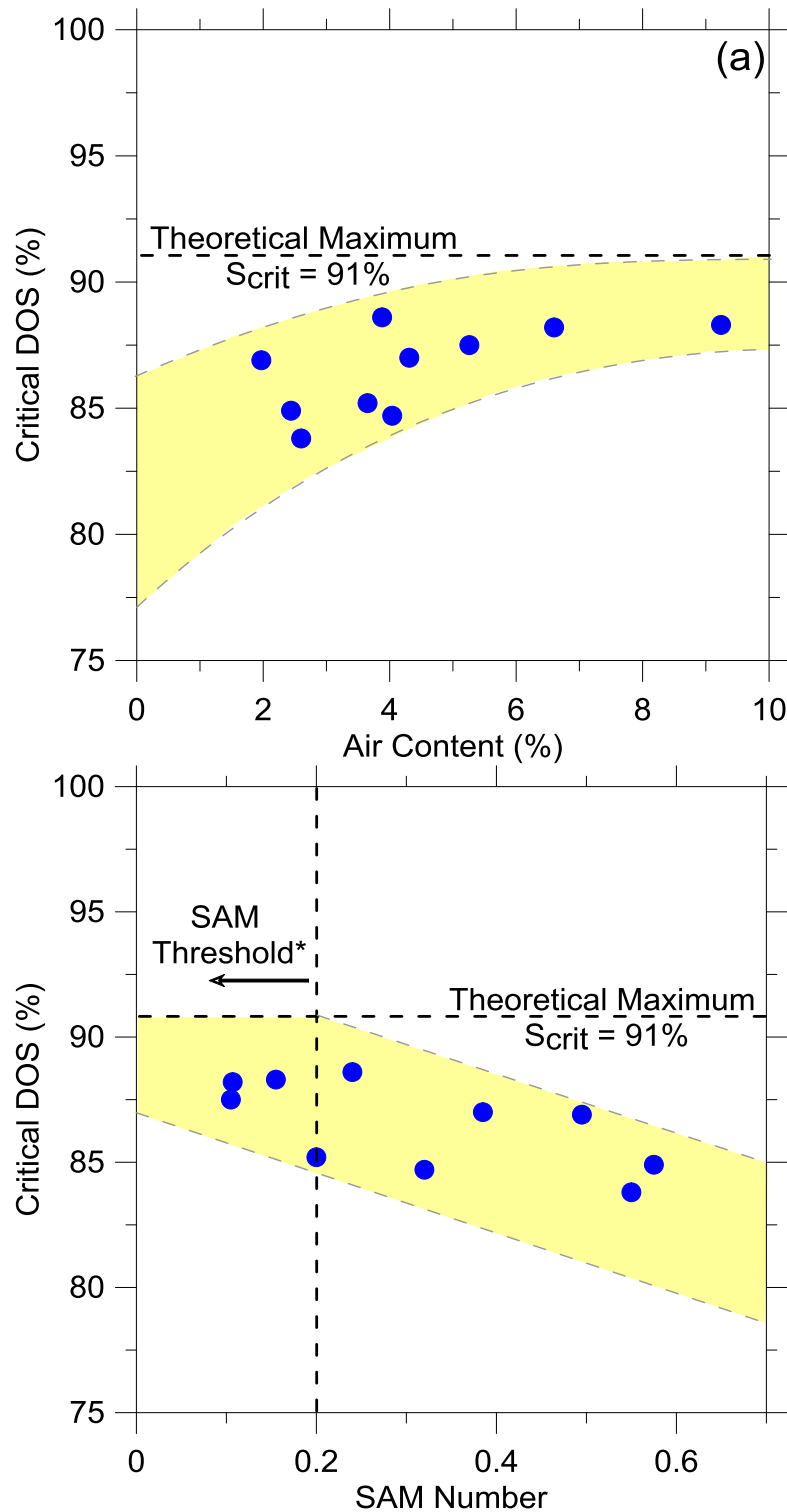
Figure 14 Projected Critical Degree of Saturation for Concrete Mixtures with a) Total Air Content and b) Air Quality (SAM Number) Using the Damage Index Following Three Freeze-Thaw Cycles
