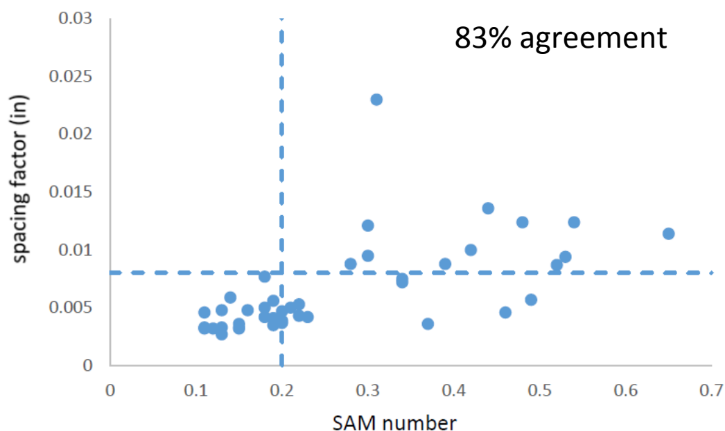
Figure 5 – Comparison of the SAM number and spacing factor for 47 field samples from Pennsylvania DOT field mixtures. A SAM limit of 0.20 and a spacing factor limit of 0.008" is shown. The results show an 83% agreement between the two methods.
