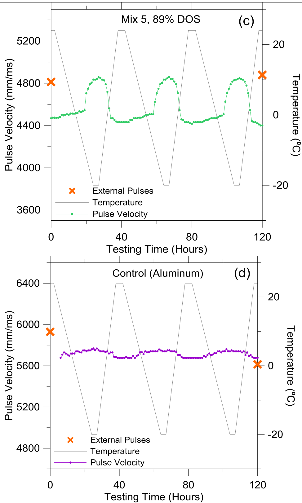
Figure 13 Wave Velocity Throughout Three Thermal Cycles for (a-c) Concrete Saturated to Three Different Degrees of Saturation Compared to (d) Control Aluminum Sample.
