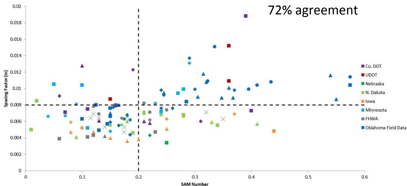
Figure 6 – Field testing data comparing the SAM number to the spacing factor for field mixtures from a number of different states with the spacing factor and SAM number compared. All mixtures were field data and they show a 72% agreement between the two methods.
