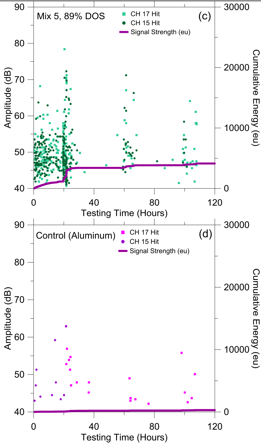
Figure 12 Acoustic Emission Hits and Cumulative Signal Strength (1eu=1nV·s) for (a) Fully Saturated (b) 94% Saturated and (c) 89% Saturated Concrete Undergoing Three Freeze-Thaw Cycles Compared to (D) an Aluminum Sample with No Freeze-Thaw Related Damage
