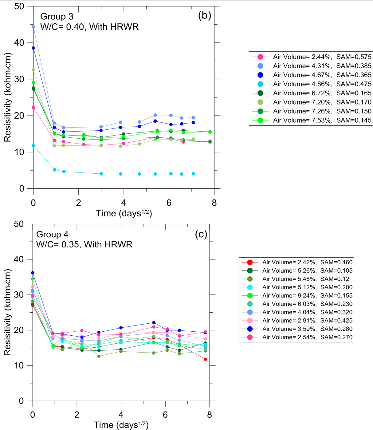
Figure 10 Sealed Resistivity and Submerged Resistivity for all 4 mixture groups
