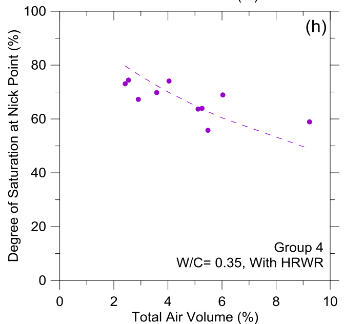
Figure 11 The Impact of Total Air Volume on (a-d) Sealed Degree of Saturation and (e-h) Nick Point Degree of Saturation Shown with Experimental Data and Theoretical Prediction
