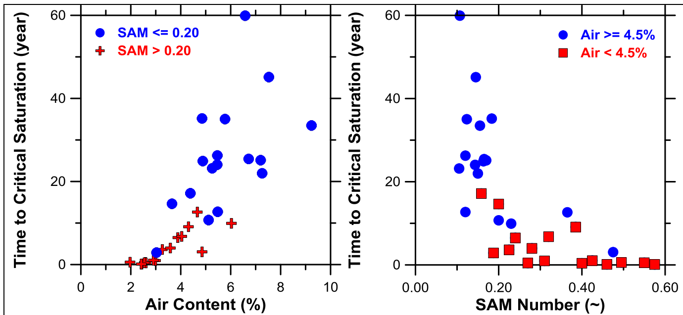
Figure 19 – Time to Saturation As A Function of Air Content and SAM Number
