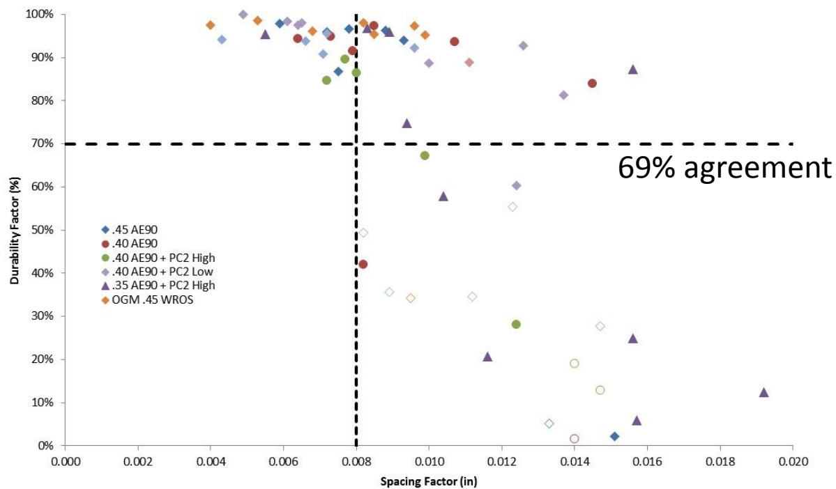
Figure 3 – A comparison of ASTM C 666 durability factor and the spacing factor. There is a 69% agreement with a spacing factor limit of 0.008”.
