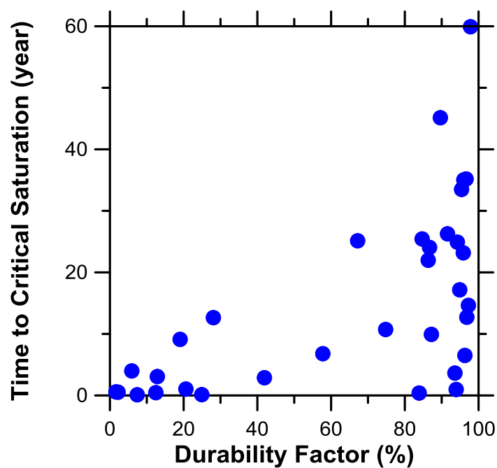
Figure 16 – Comparison of the time to reach critical saturation (as determined from measured absorption and measured secondary sorptivity) as a function of measured durability factor.
