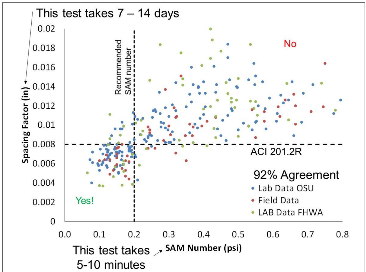
Figure 1 – A combination of OSU lab data, Oklahoma field data, and FHWA lab data that compares the SAM to the spacing factor. There is a 92% agreement between the data sets.
