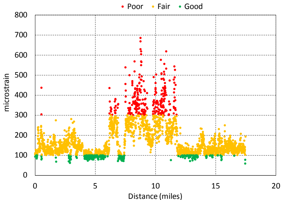
Figure 19. Estimated tensile strain at bottom of asphalt layer on SR12.
