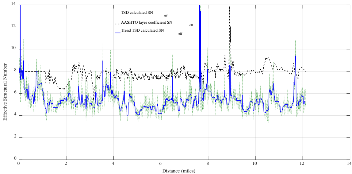
Figure 17 Example of calculated effective structural number on I680 north tested in 2014 (see Figure 18 or following link https://goo.gl/maps/6ZADtjriGeA2 )
