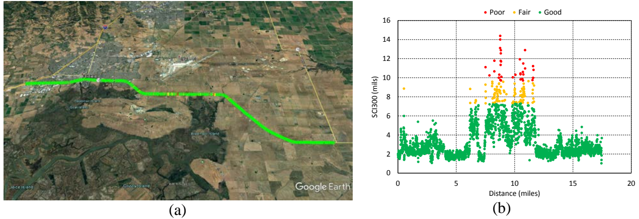
Figure 14. Identified Strong (green) and Weak (red) sections on SR12 based on thresholds obtained from Table 2: (a) Google Earth plot (© 2016 Google); (b) figure plot
