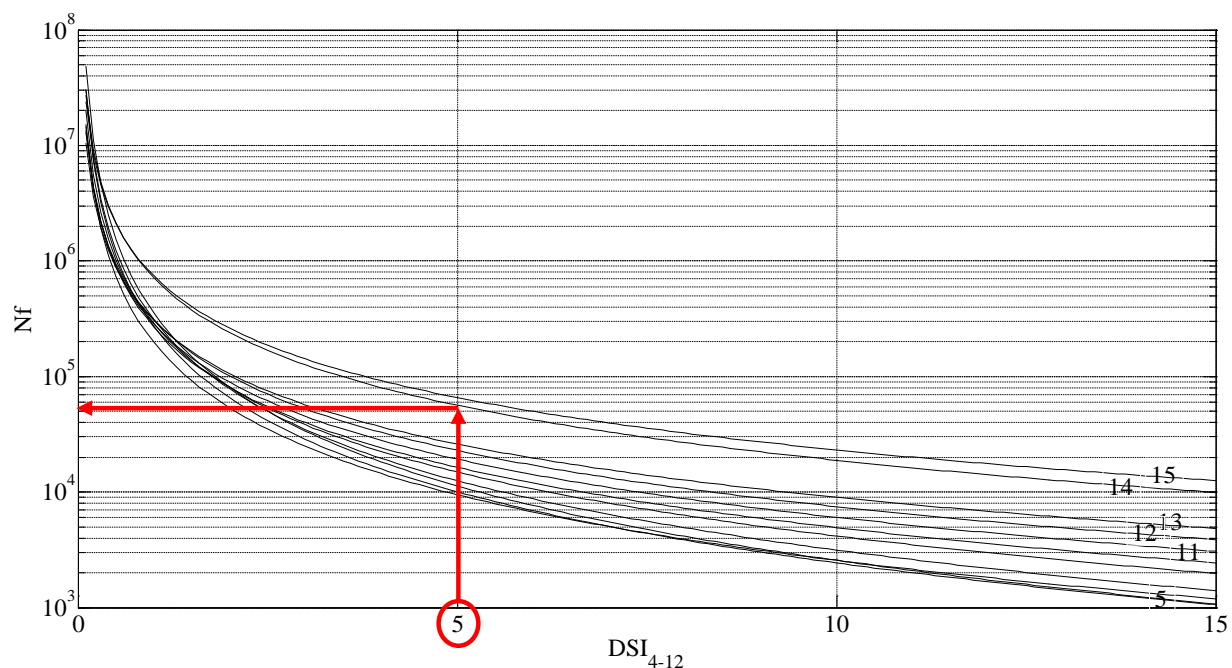
Figure 21. Fatigue life curves for TSD DSI.
