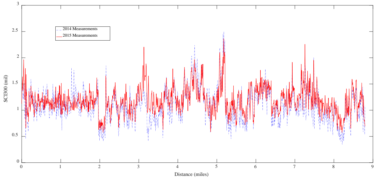
Figure 11. Temperature corrected repeated TSD tests on Jackson Road west
