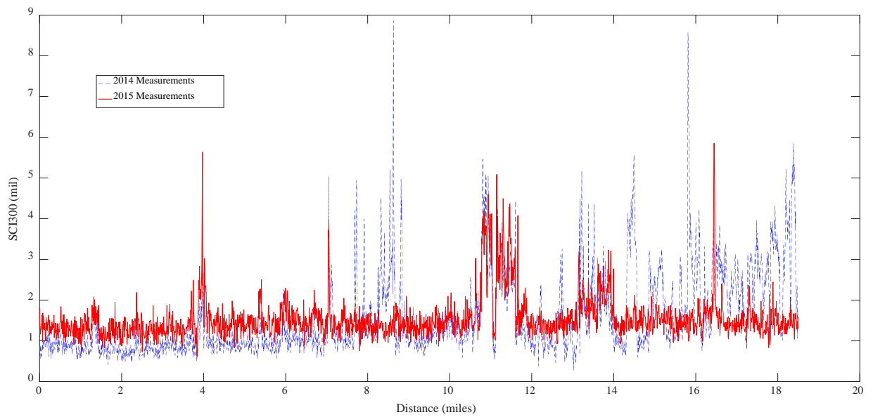
Figure 12 Temperature corrected repeated TSD tests in 2014 and 2015 on R99 South (Golden State Highway South) https://goo.gl/maps/UisyVwrZbZ72
