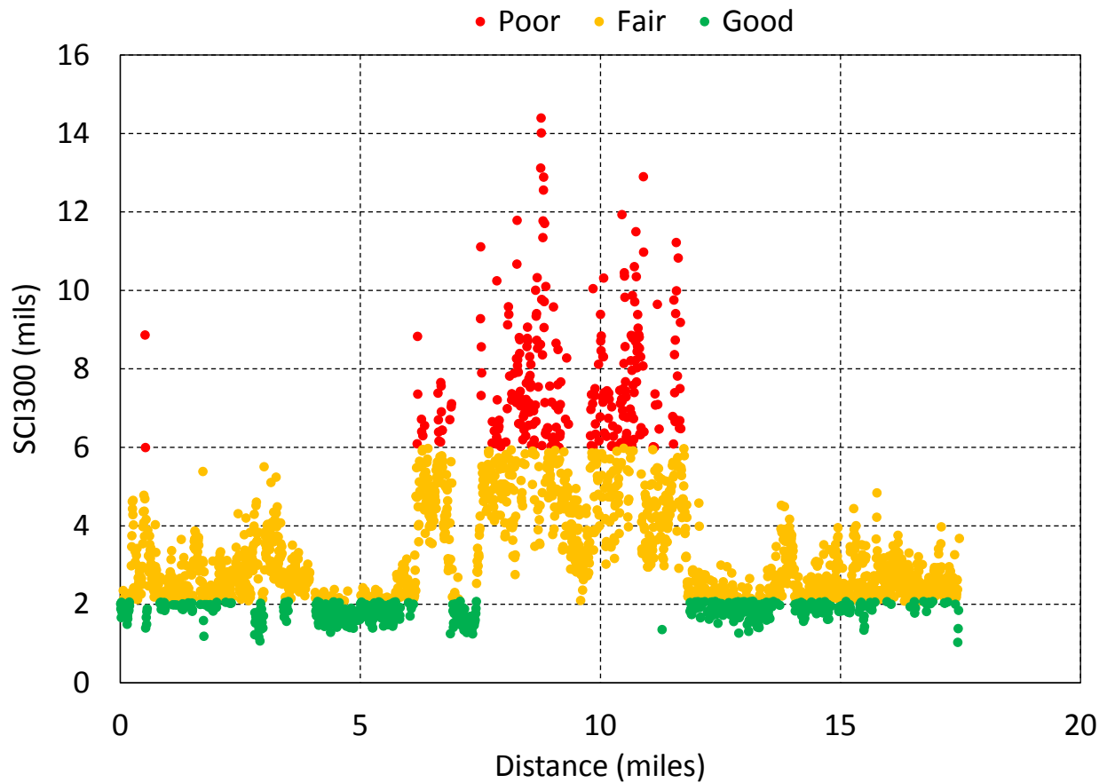
Figure 15 Classification of condition on SR12 based on percentile: 25 th percentile and lower represents good condition and 90 th percentile and higher represents poor condition
