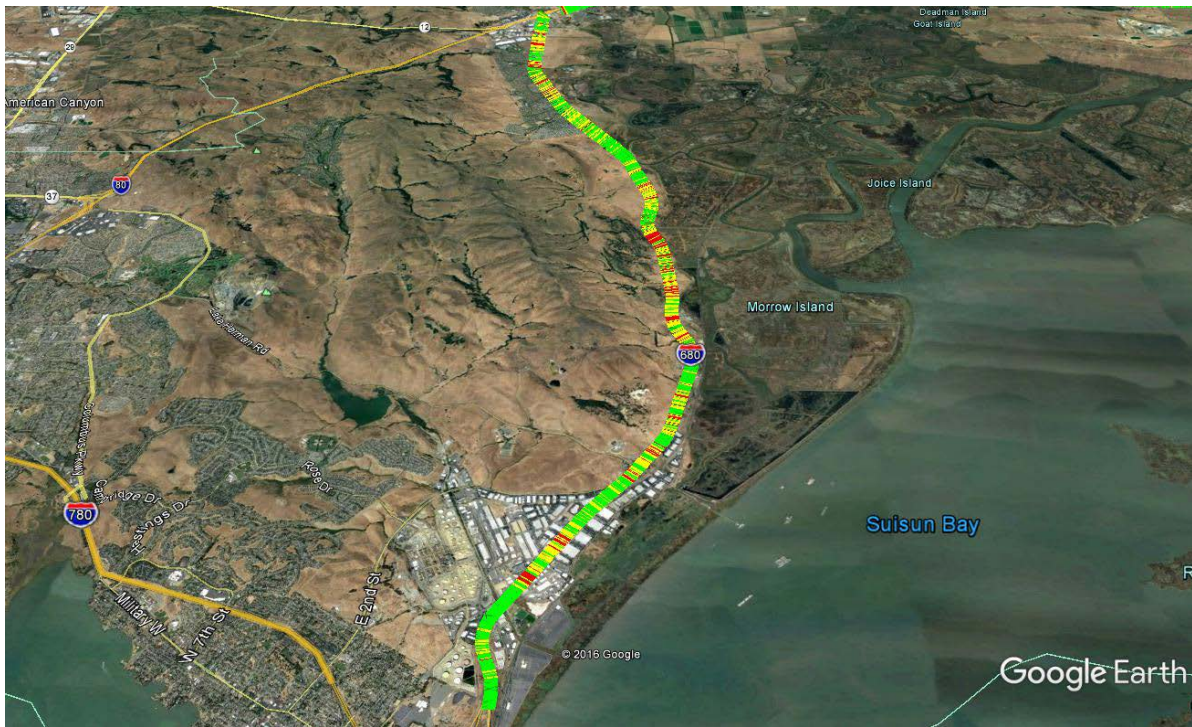
Figure 6. Detail example of pavement condition: I680 tested in 2014 (© 2016 Google Image Landsat / Copernicus).
