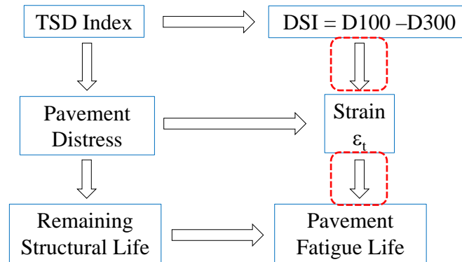
Figure 20. Link between DSI and estimated pavement fatigue life.
